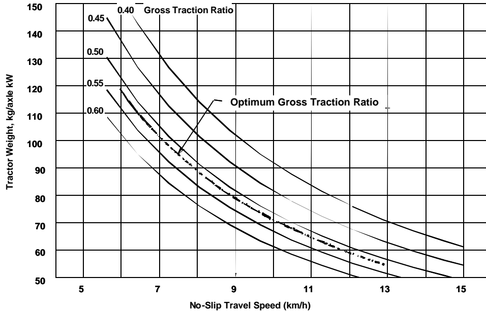
Figure 49. Weight-speed-power relationship.
