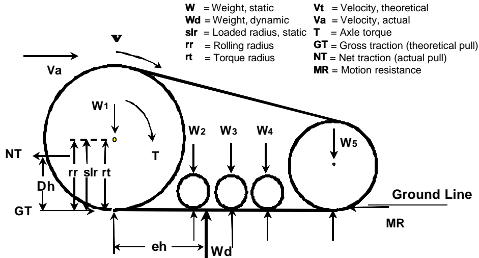
Figure 4. Belt drive.
