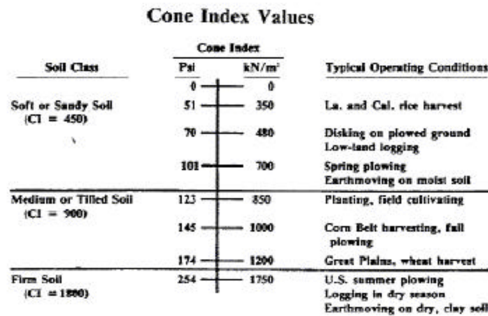
Figure 45. Typical cone index values (from Brixius, 1987).
