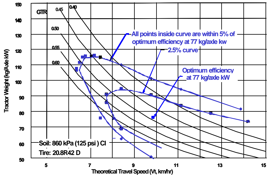
Figure 50. Optimum tractor weight and sensitivity analysis (John Deere 8870 4WD).
