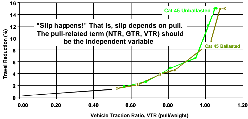
Figure 9. Nebraska test performance comparison with VTR as independent variable.
