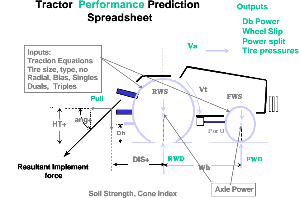
Figure 46. Tractor diagram for tractor performance prediction spreadsheet (performance calculation).
